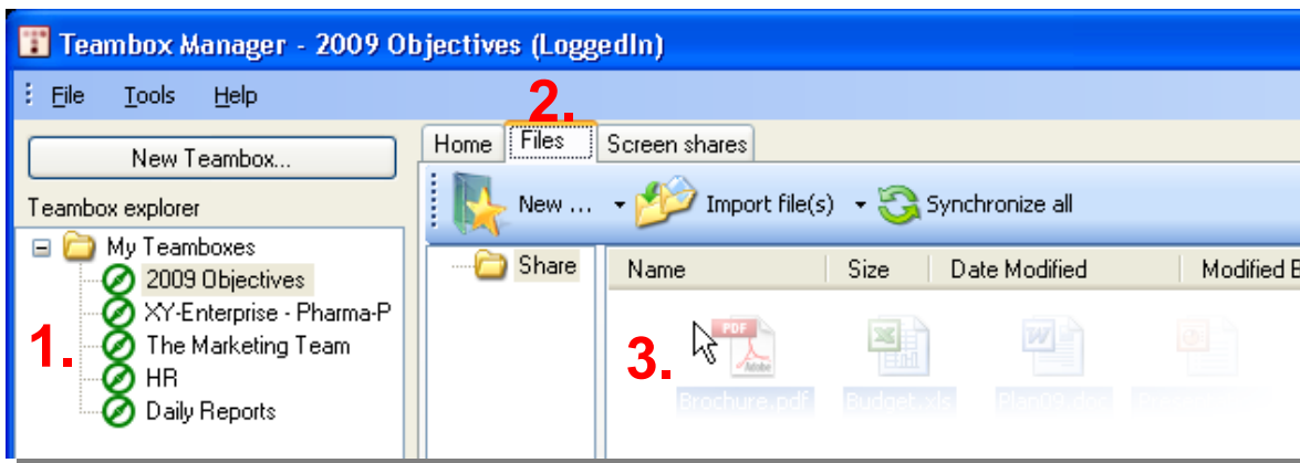
Sharing Files
